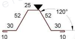
ST 076 - T45 trapézelem T= 208mm
